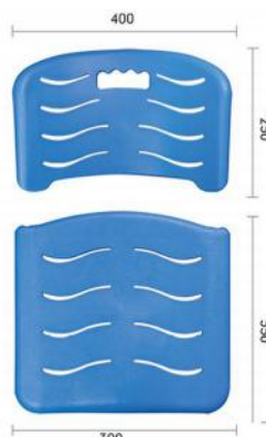
Z F-8017 400x250mm 390x350mm
