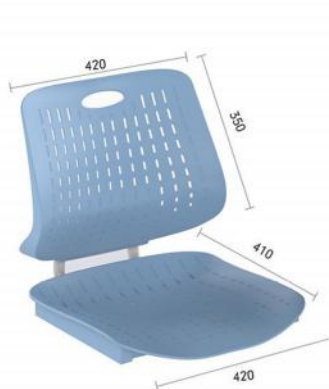
Z F-8529 420x350x50mm 420x410x50mm
